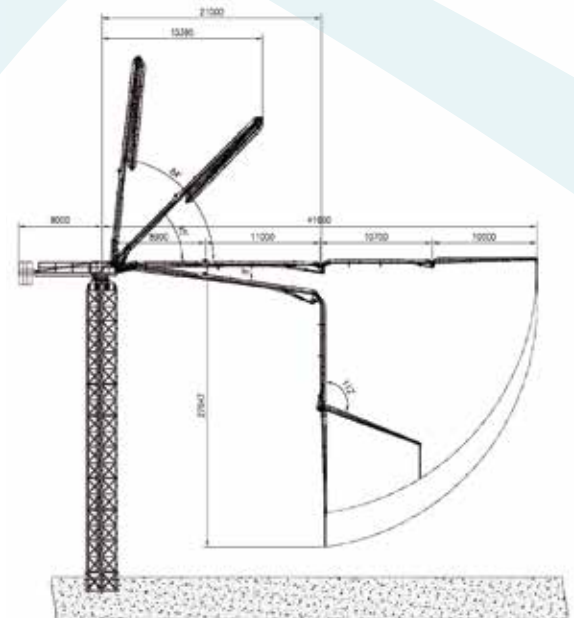
EPB42 WORKING DIAGRAM
